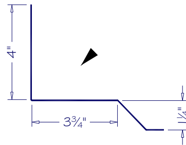
SIDE WALL SW-02
