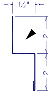
GABLE DIVIDER GB-03
