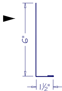
FASCIA FC-02
