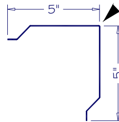
OUTSIDE CORNER OSC-02
