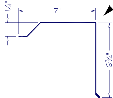
GABLE GB-04
