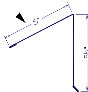
PEAK CAP PC-03
