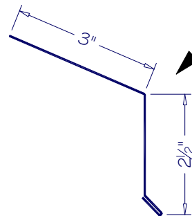
EAVE EV-02
