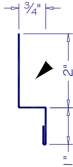
GABLE DIVIDER GD-02
