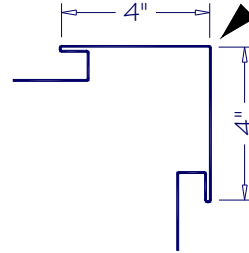
OUTSIDE CORNER OSC-04
