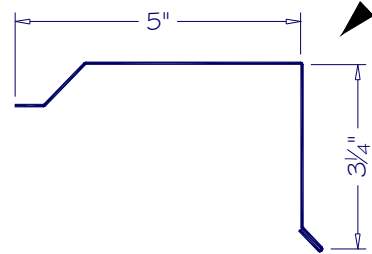
GABLE GB-02
