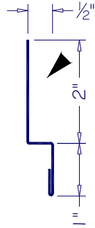
GABLE DIVIDER GD-01
