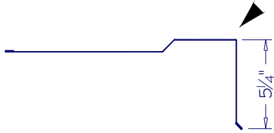
PROW GABLE GB-P3
