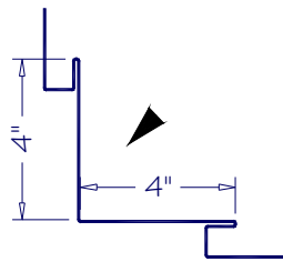
INSIDE CORNER ISC-03
