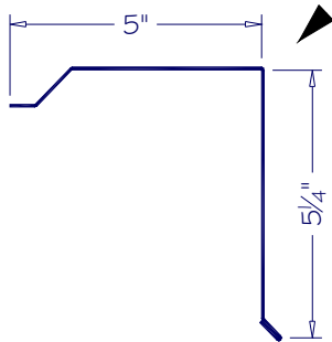
GABLE GB-03
