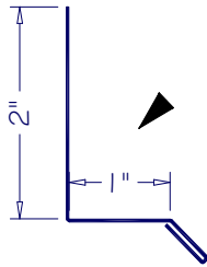
BASE BF-01
