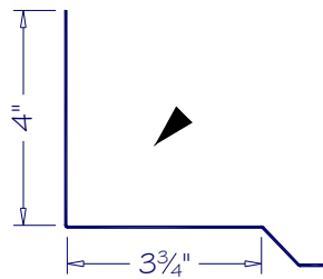
SIDE WALL SW-01
