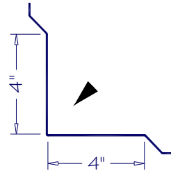
INSIDE CORNER ISC-02
