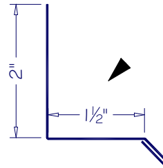
BASE BF-02
