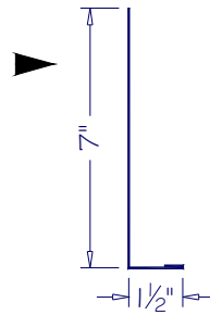
FASCIA FC-03
