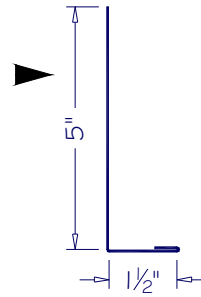
FASCIA FC-01
