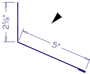
END WALL EW-01
