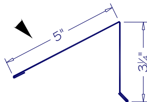
PEAK CAP PC-02
