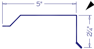
GABLE GB-01
