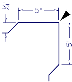
OUTSIDE CORNER OSC-05
