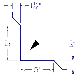
INSIDE CORNER ISC-05
